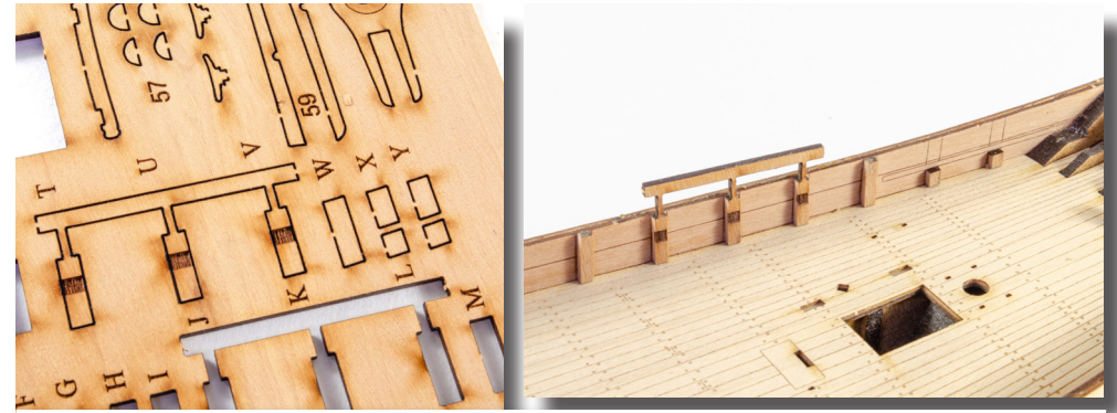
102. We now have three more timberheads (T, U, V) on a single part, and W, X, and Y as separates. Remove these from the 1.5mm wood sheet. Glue into position after the previous timberheads. Note that you will only glue into position the lower parts of X & Y at this stage.
