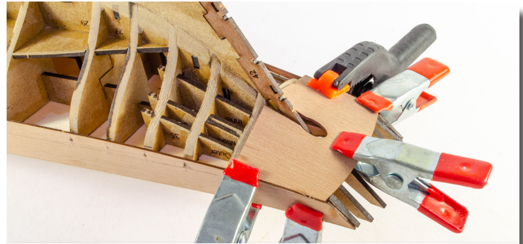
59. On the prototype, we found that soaking the part for 30 mins in hot water, and then clamping in place until dry, really helped with fitting. If you soak this part, you must leave it to dry for at least 12hrs for it to regain its original shape. Pear wood does expand quite a lot when it gets wet. Once dry, glue and pin in place.
