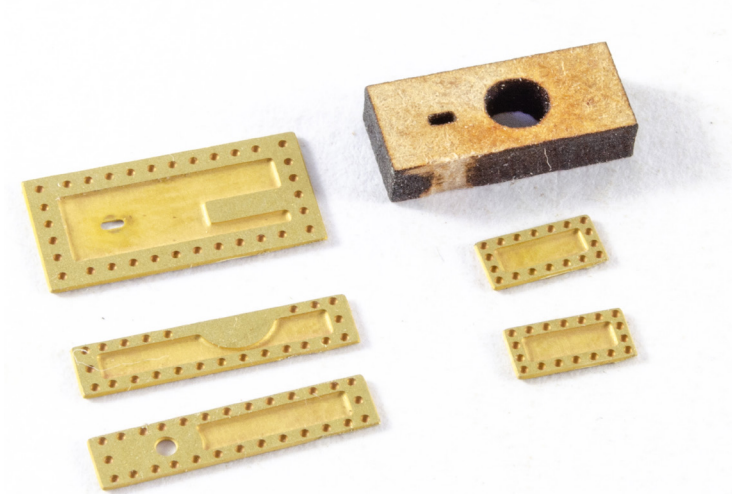
173. You will now need the very last MDF part, #121. This will form the core of the head assembly. From the PE sheet, also remove parts #PE41 thru #PE44.
