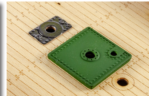
137. Glue these parts together and prime. We painted this green to match the outer bulwarks. Glue the assembly to the deck. After painting, also glue #PE-35 to the deck.
