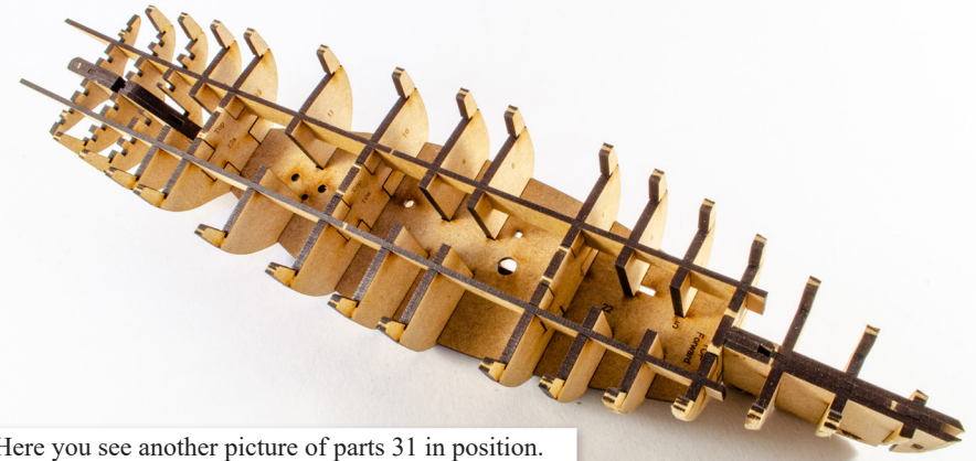
31. Here you see another picture of parts 31 in position.
