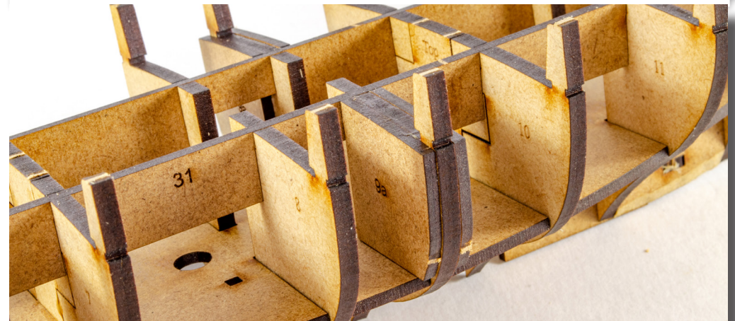
33. Glue these into place on either side of bulkhead #9, so they sit on the lower deck and against parts 31 that you just fitted.
