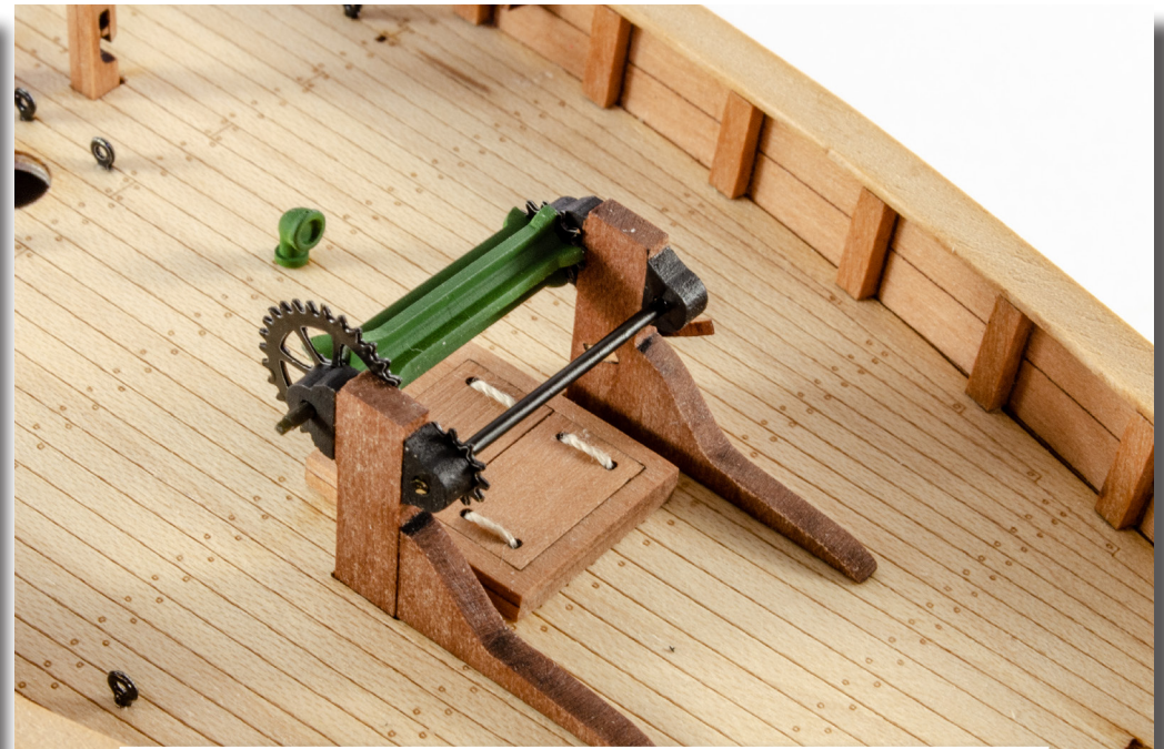
194. The windlass can now be installed in position in the slots on the deck.
