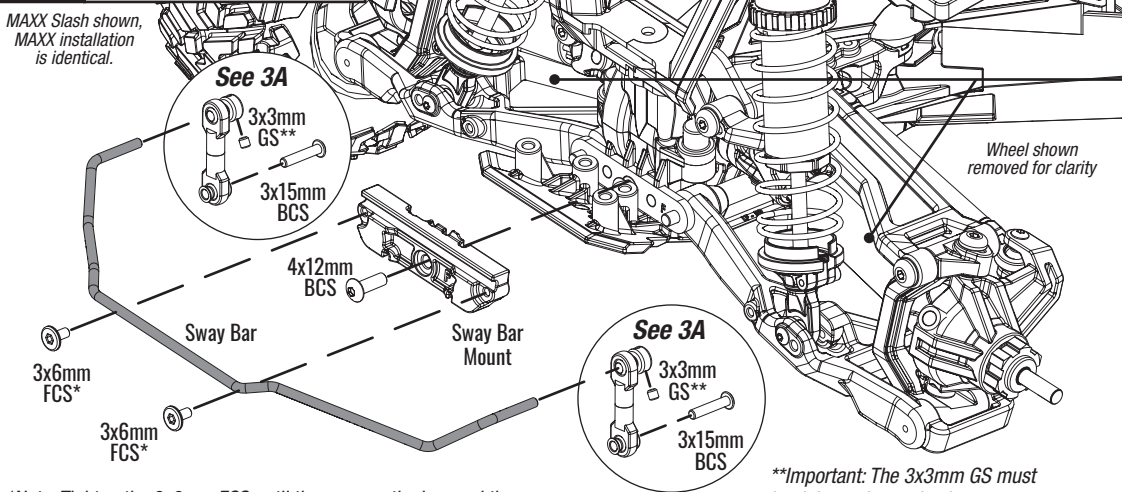
Fig 3 Front Sway Bar Install
