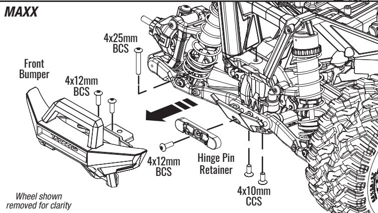
Fig 3 Front Sway Bar Install
