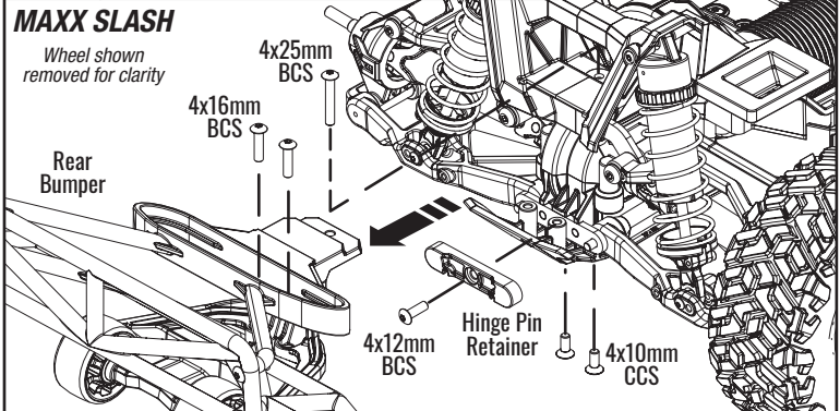
Fig 2 Rear Hinge Pin Retainer Removal
