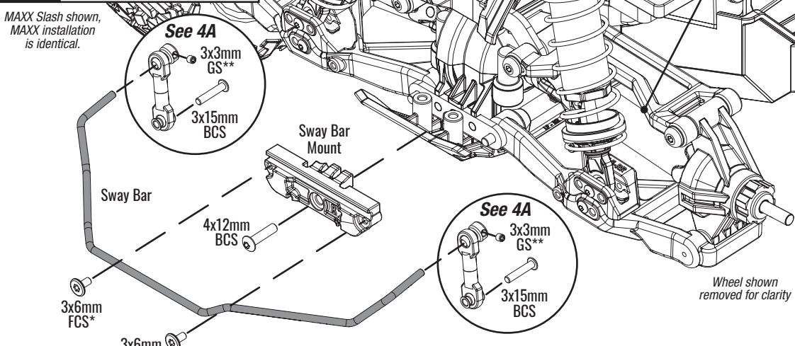
Fig 4 Rear Sway Bar Install
