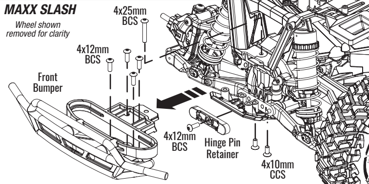
Fig 1 Front Hinge Pin Retainer Removal
