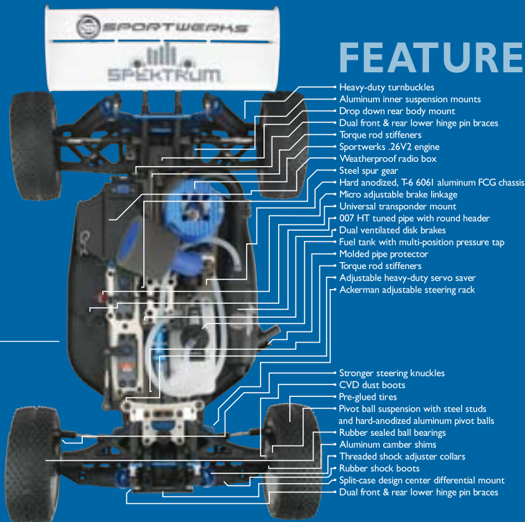
SWK1225 Turmoil RTR 1/8 4WD BUGGY
